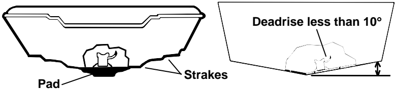
Left, vee pad hull; right, vee hull. A pod style transducer is shown here, but the principle is the same for Skimmers inside a hull.
