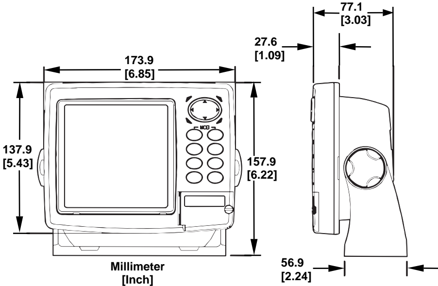
Front view (left) and side view (right) showing dimensions of the X100C or X105C DF when mounted on gimbal bracket.
