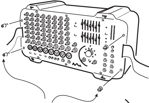
remove 4 rack bolts
